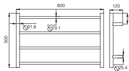
HTR500X800-4 Heater Towel Rail
