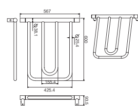
HTR565X600-4 Heater Towel Rail
