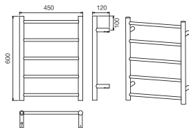
HTR600X450-5 Heater Towel Rail
