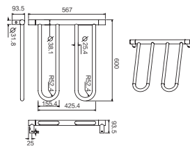
HTR567X600-4 Heater Towel Rail
